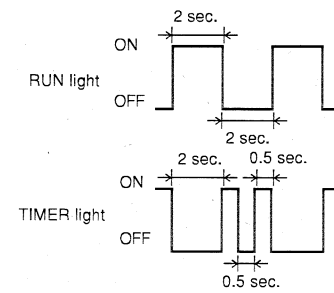
Display in DRED mode during Defrost operation
